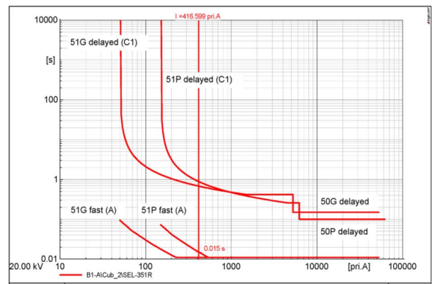
Fig. 8. Nuisance feeder tripping when DG is present.
