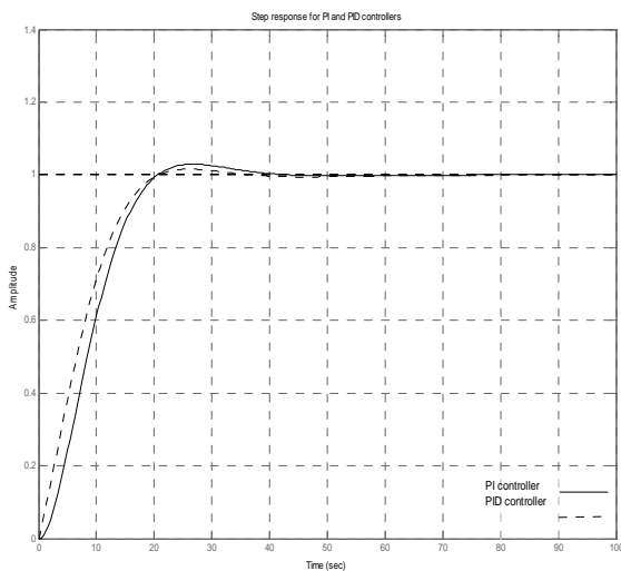
Fig. 9 The comparison between PI and PID controller
