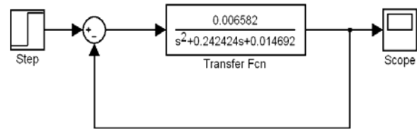
Fig. 4 Simulink block diagram of the system without controller
