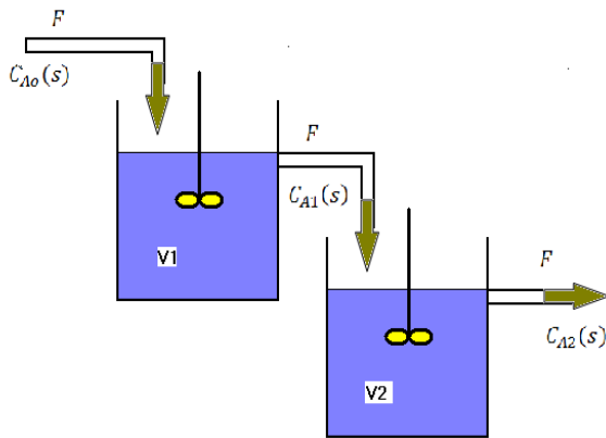
Fig.1 The simple concentration process control
