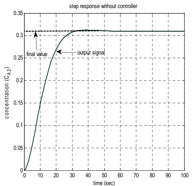
Fig. 5 Step response of system without controller
