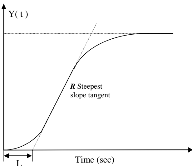
Fig. 6 Process step response
