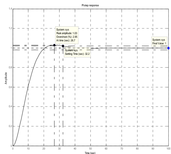
Fig. 7 The output response for PI controller
