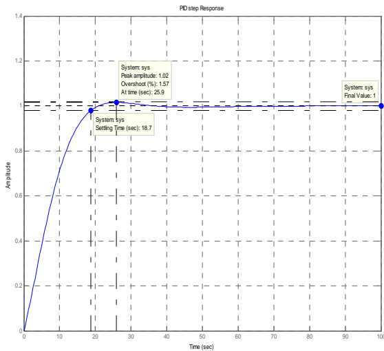
Fig. 8 The output response for PID controller
